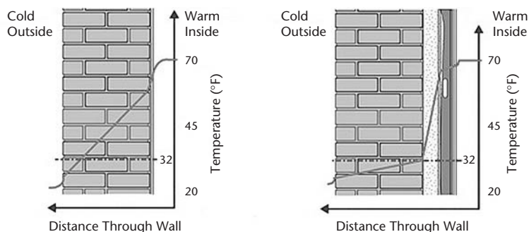
FIGURE 5. Changing temperature gradient due to interior insulation.
