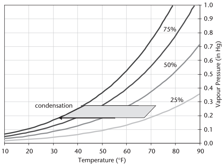
FIGURE 7. Temperatures at which condensation can occur.
