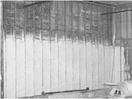
FIGURE 9. Field installation of spray foam. (Photo courtesy of Icyne®.)
