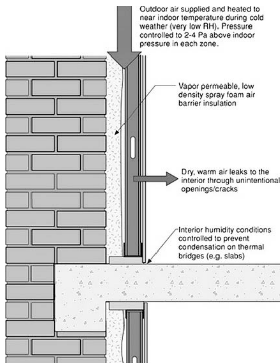
FIGURE 11. Concept drawing of pressure controlled interior retrofit.
