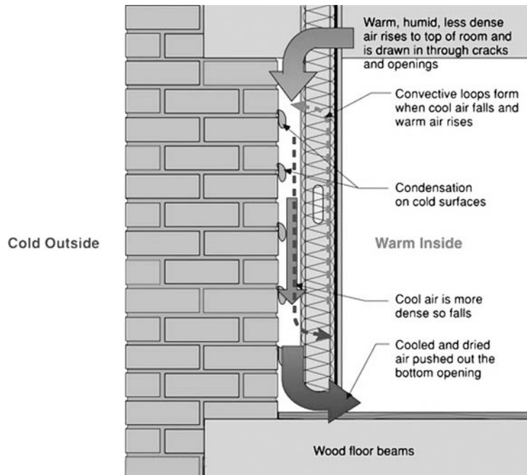
FIGURE 6. Concept drawing of stud and batt interior retrofit.
