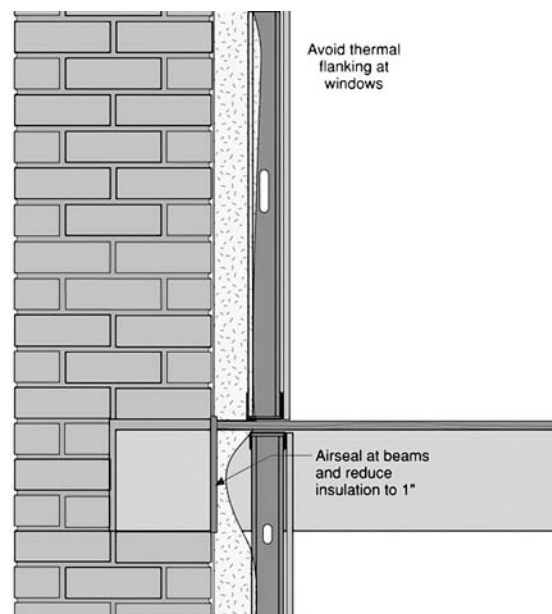
FIGURE 8. Concept drawing for spray-foam retrofit.
